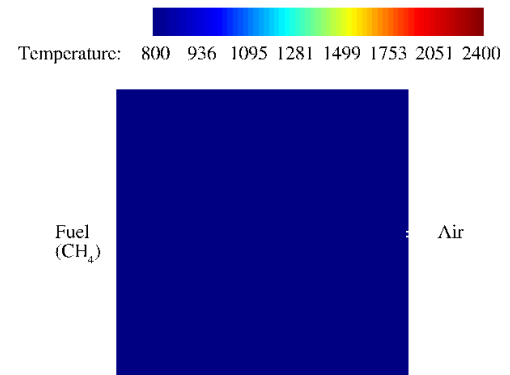
Counter Flow Flame
